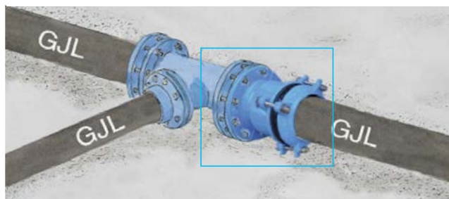
FIG. 3 Synoflex flange adaptor
