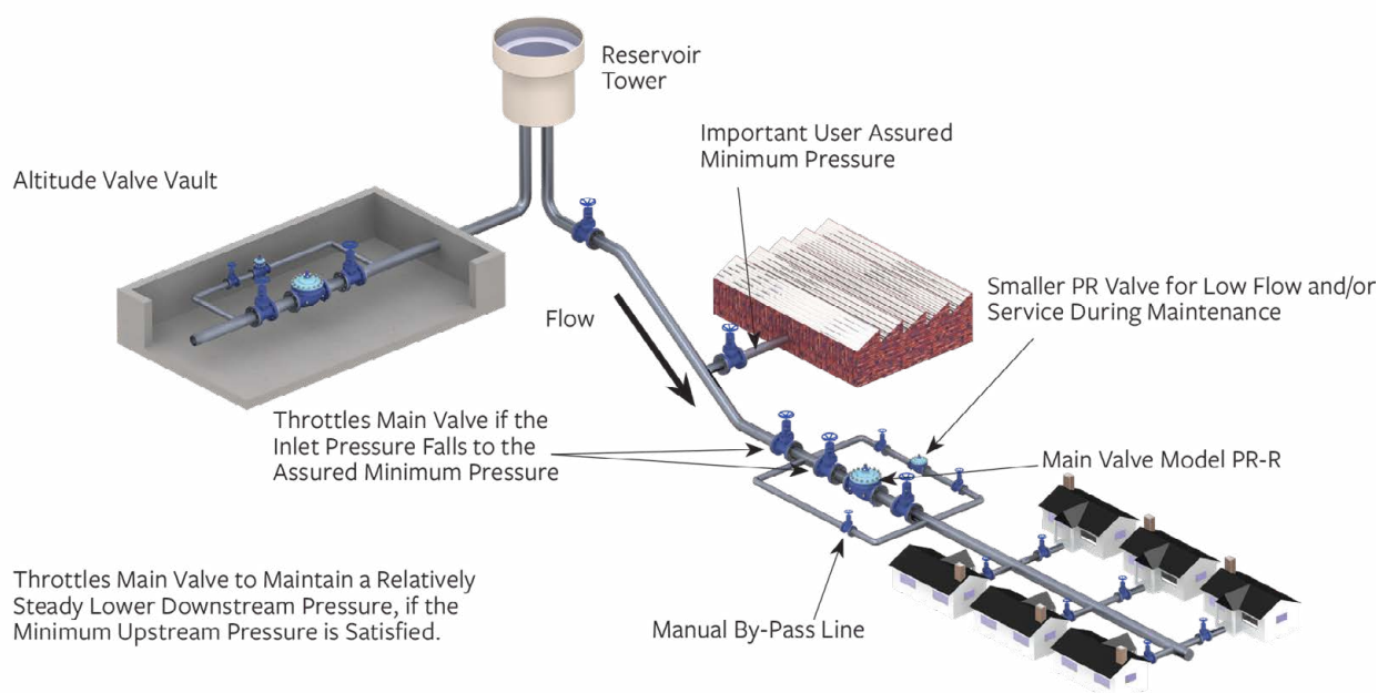
FIG. 1 Typical Application
